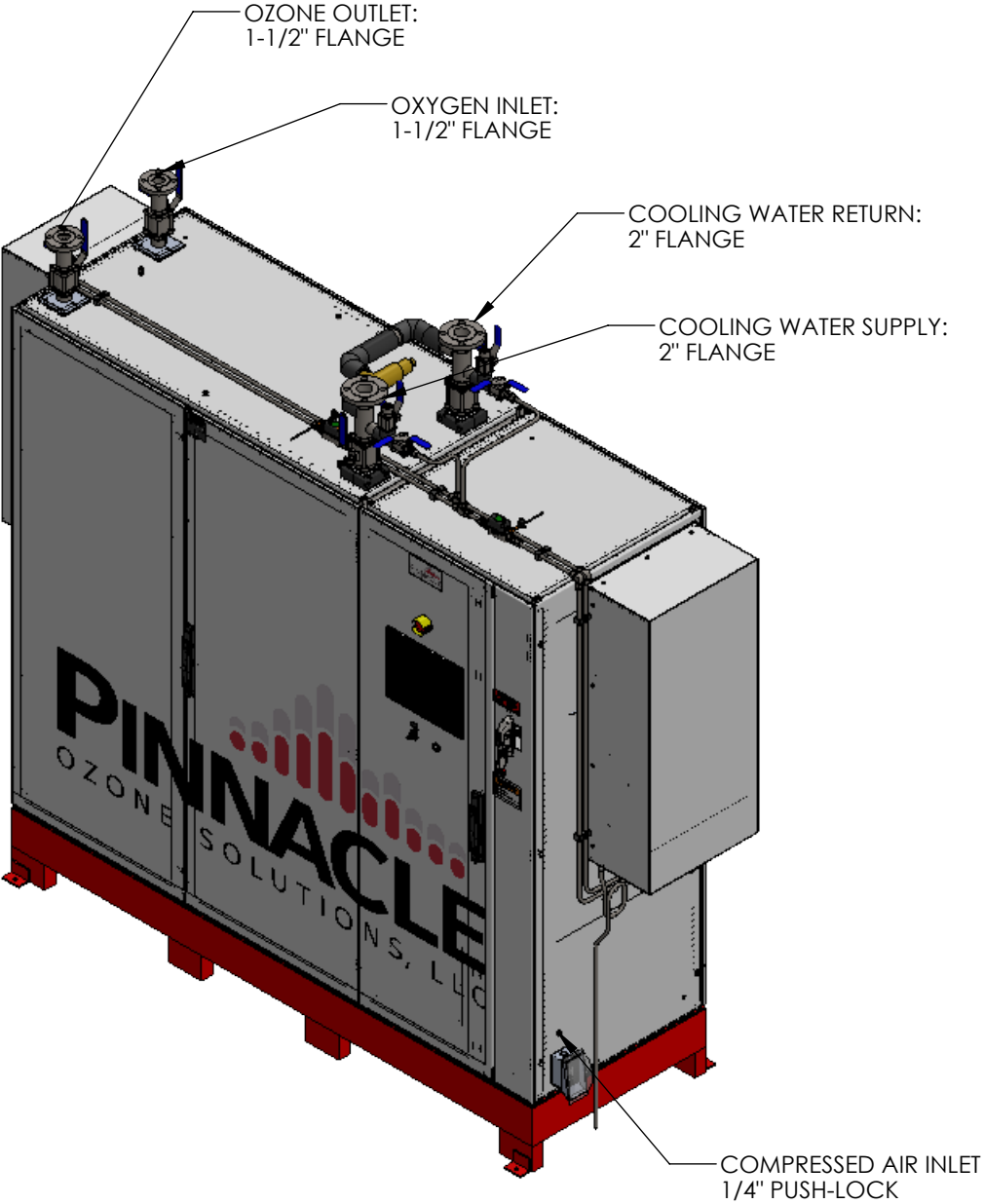
3D VIEW 0790-1000 OZONE GENERATOR ASSEMBLY, 36X
