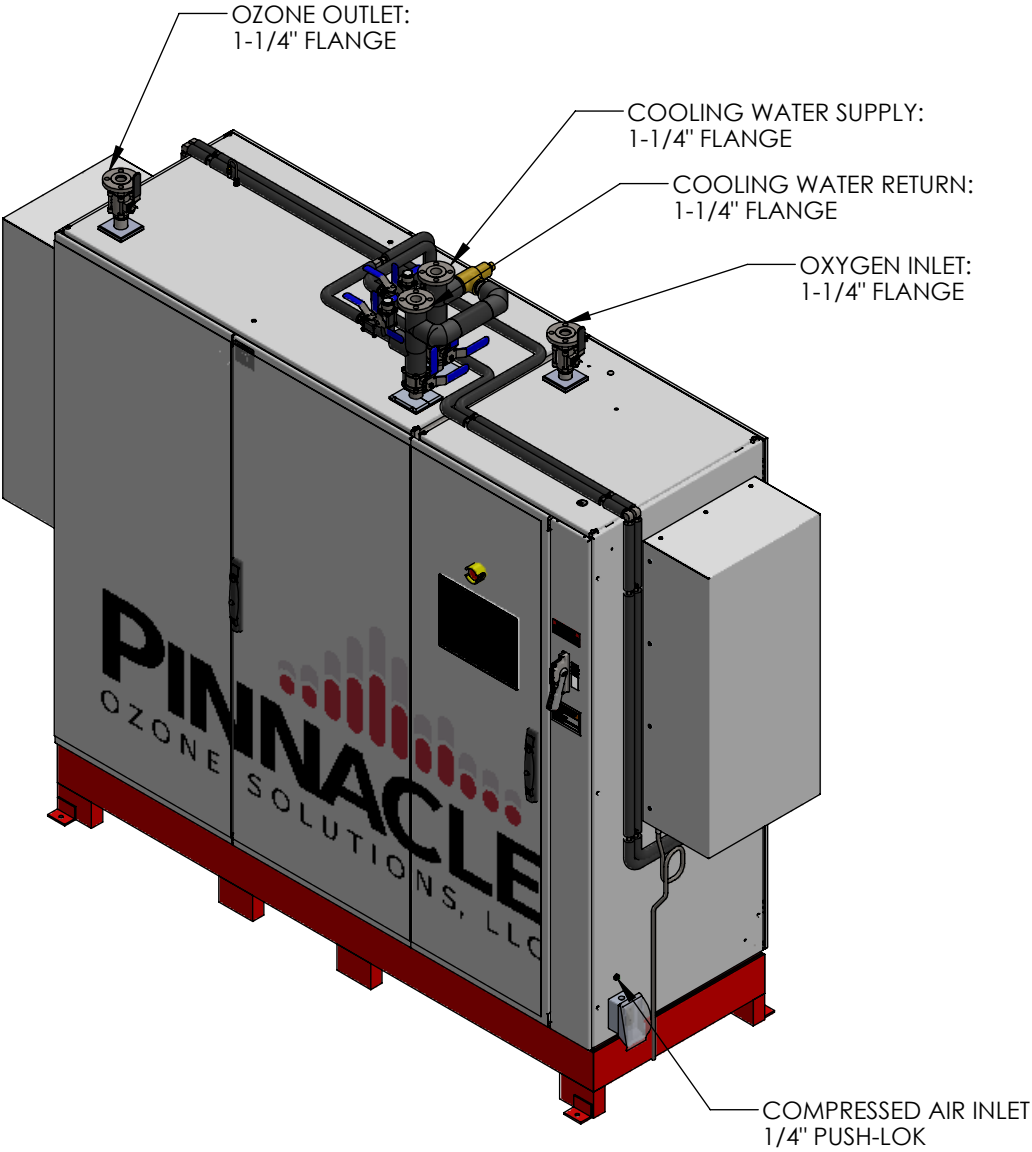
3D VIEW 0780-1000 OZONE GENERATOR ASSEMBLY, 30X
