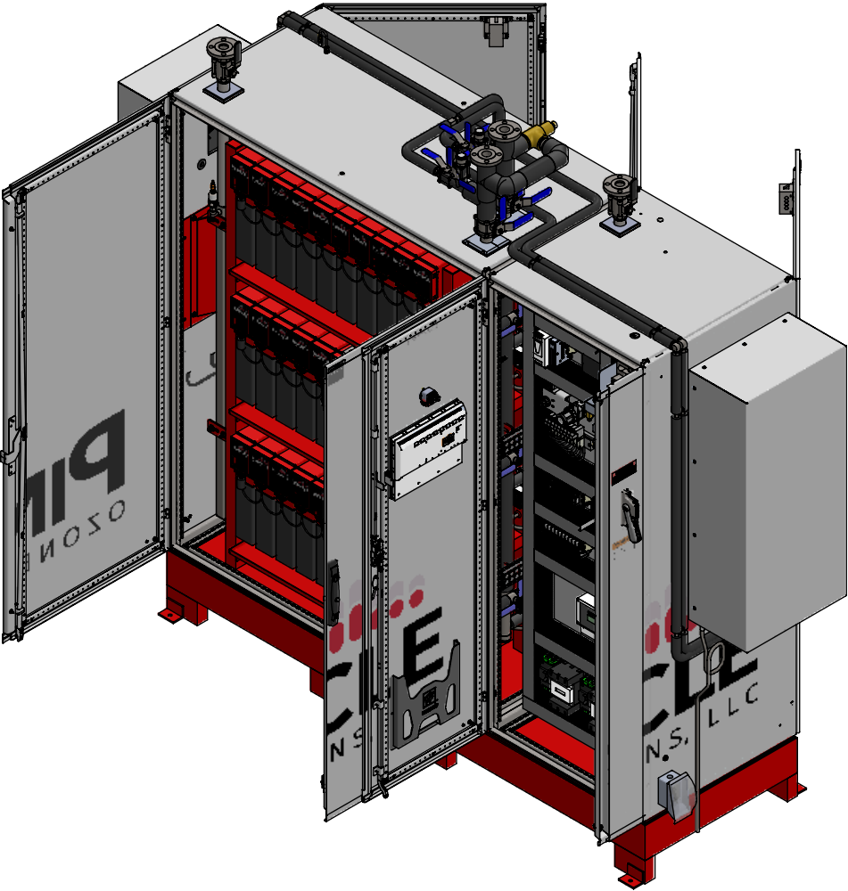
3D VIEW 0780-1000 OZONE GENERATOR ASSEMBLY, 30X (DOORS OPEN)
