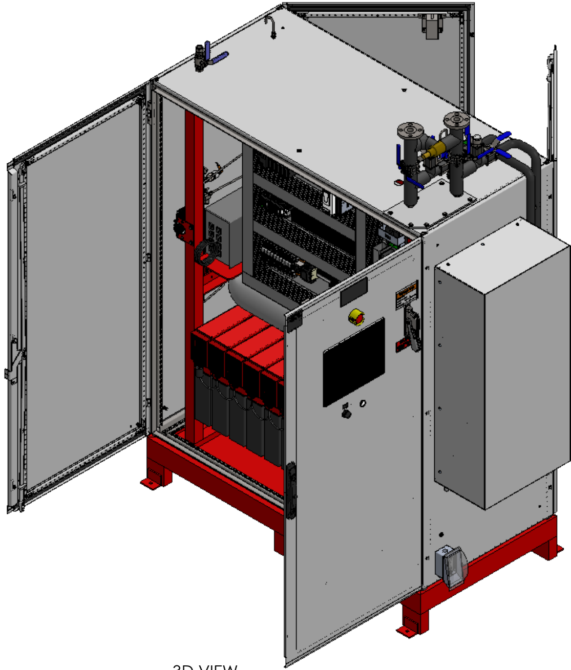
3D VIEW 0740-1000 ASSEMBLY, 12-UP OZONE GENERATOR (DOORS OPEN)
