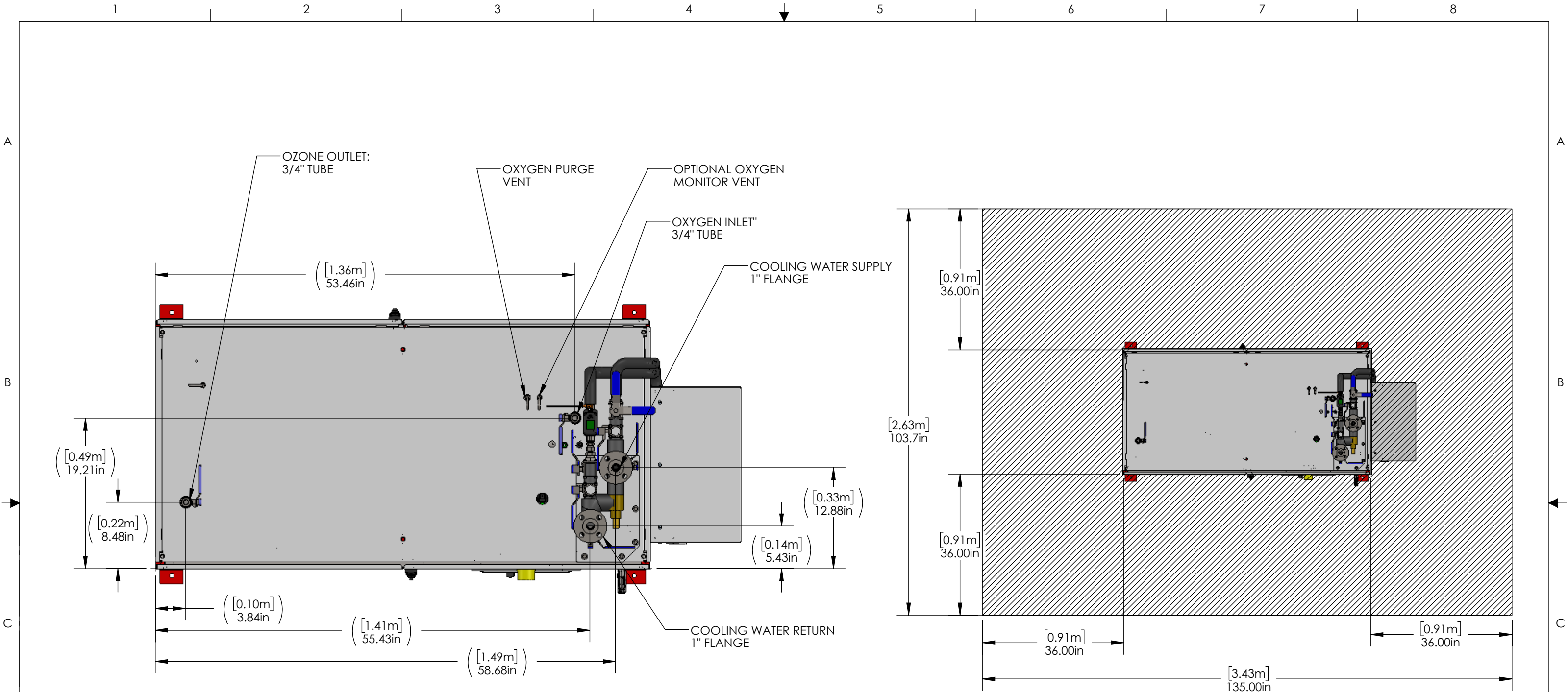
TOP VIEW (RECOMENDED CLEARANCE) 0740-1000 ASSEMBLY, 12-UP OZONE GENERATOR
