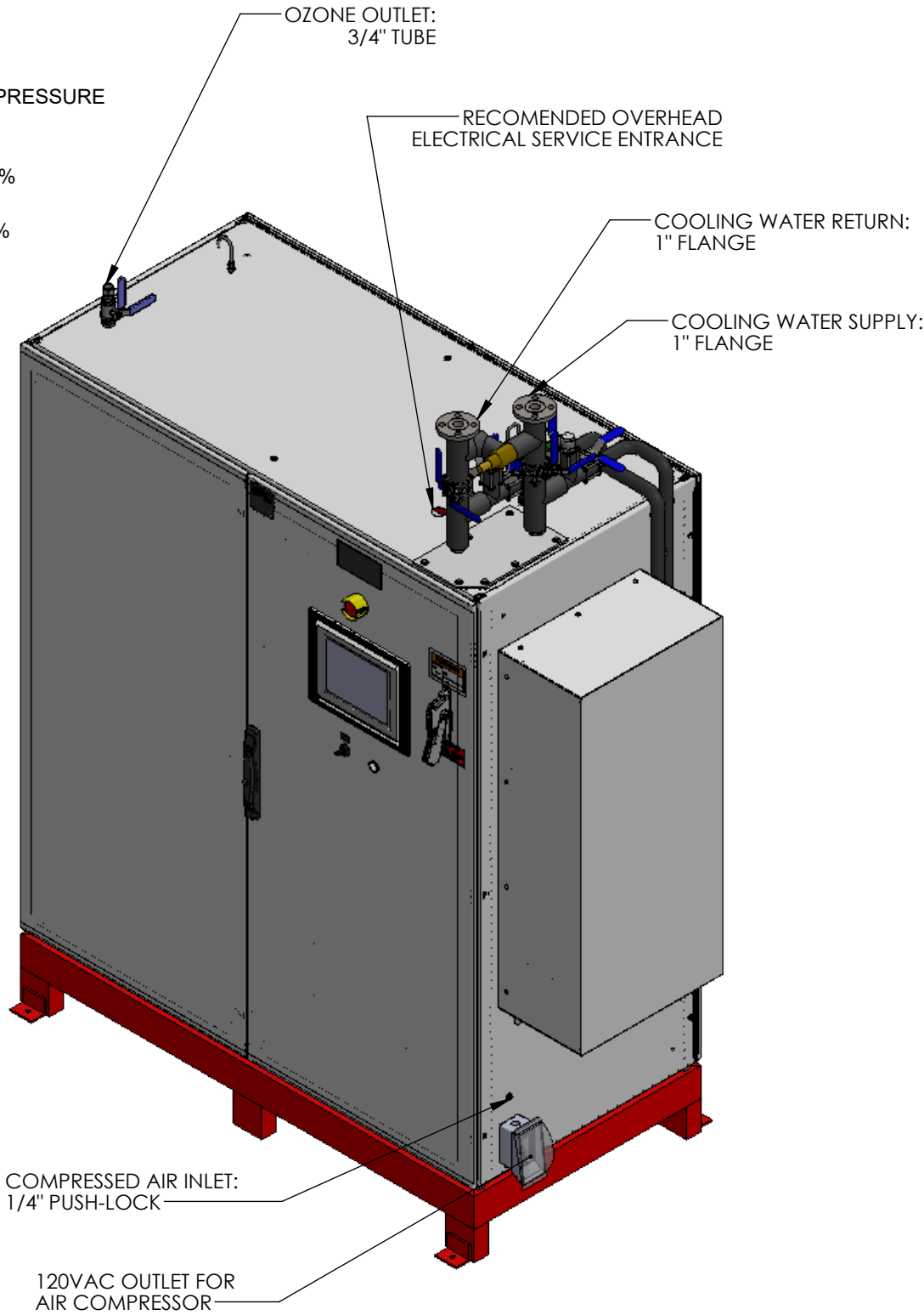
3D VIEW 0740-1000 ASSEMBLY, 12-UP OZONE GENERATOR
