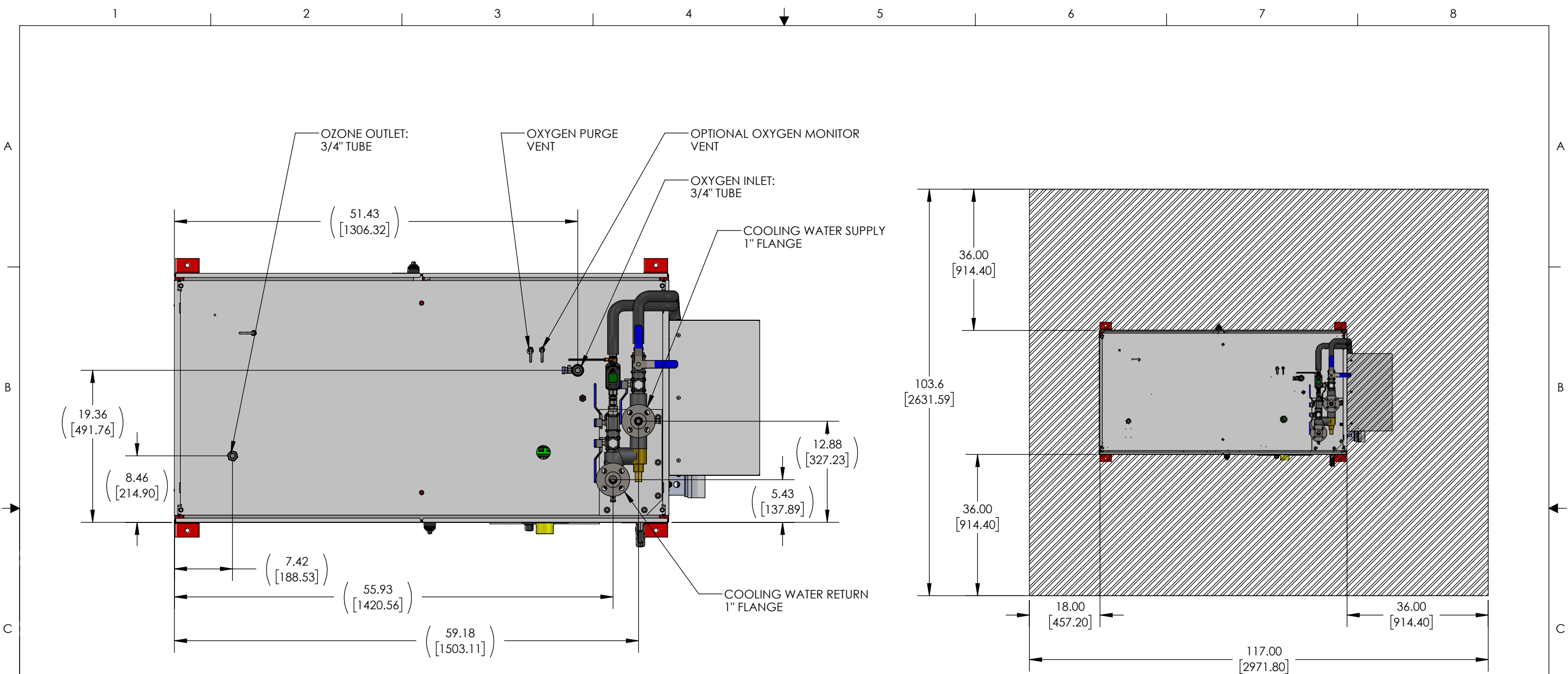
TOP VIEW (RECOMENDED CLEARANCE) 0760-1000 OZONE GENERATOR ASSEMBLY, 10X
