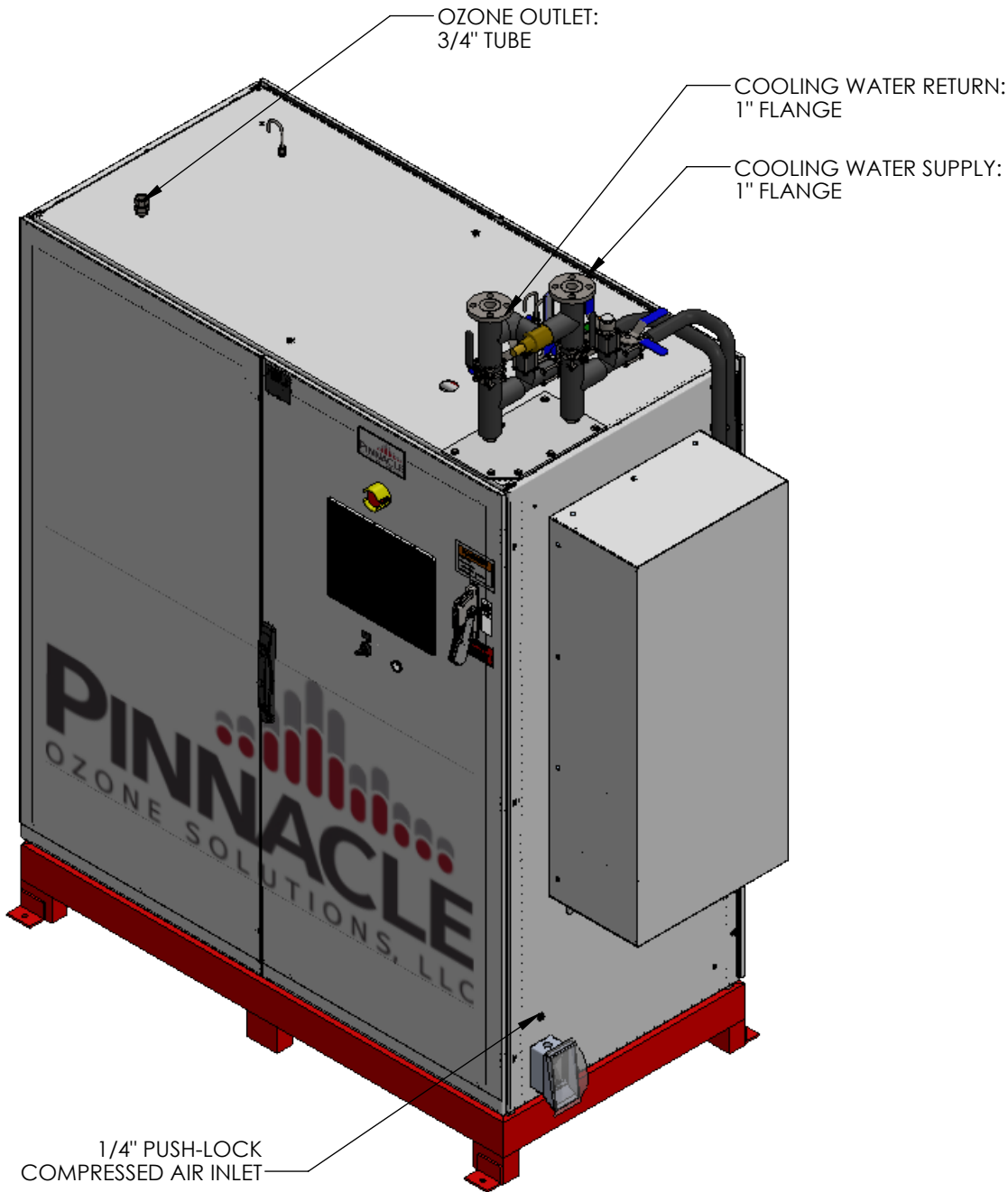
3D VIEW 0760-1000 OZONE GENERATOR ASSEMBLY, 10X
