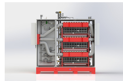
Rear view cutaway of Zenith 30X ™
