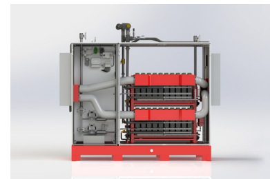
Front view cutaway of Zenith 20X
